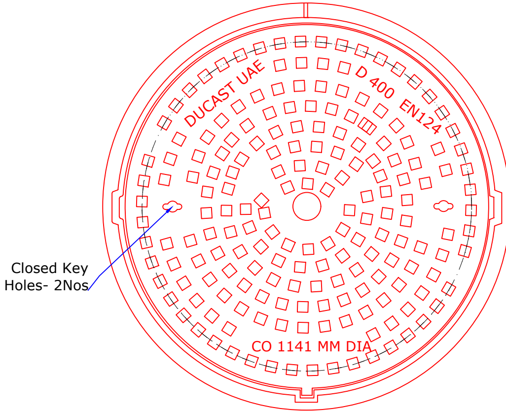
Plan View of Cover & Frame
