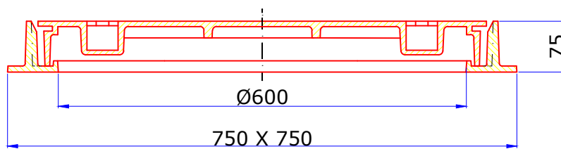
Sectional View of Cover & Frame
