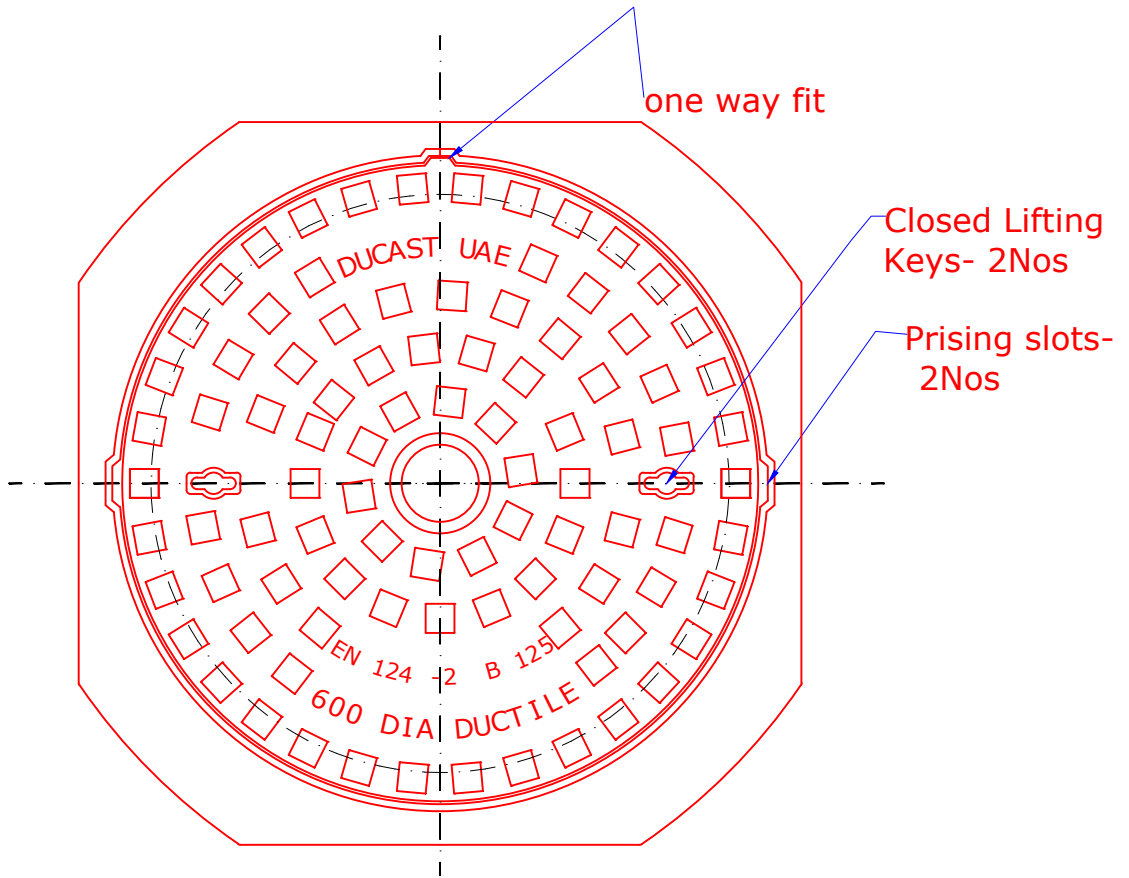
Plan View of Cover & Frame
