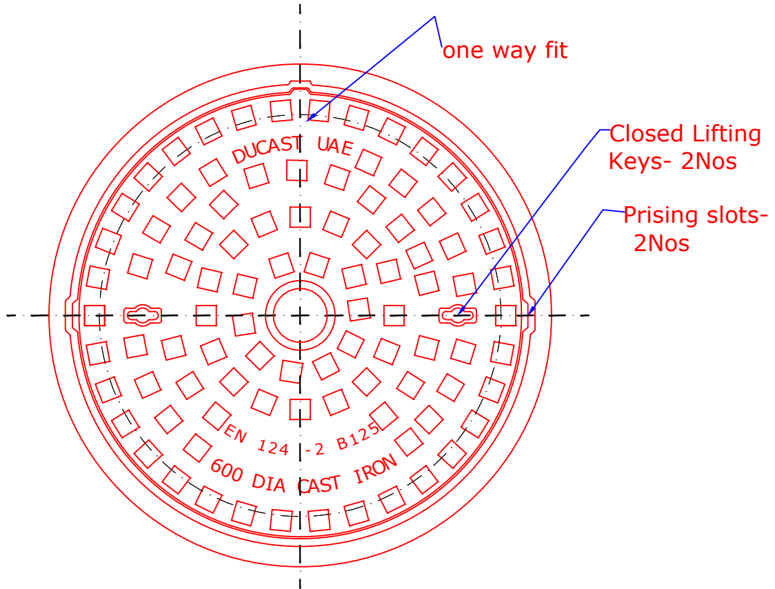
Plan View of Cover & Frame
