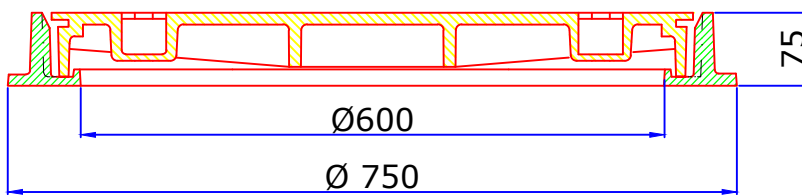
Sectional View of Cover & Frame
