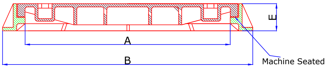
SECTIONAL VIEW
