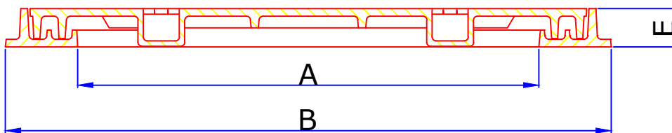
SECTIONAL VIEW
