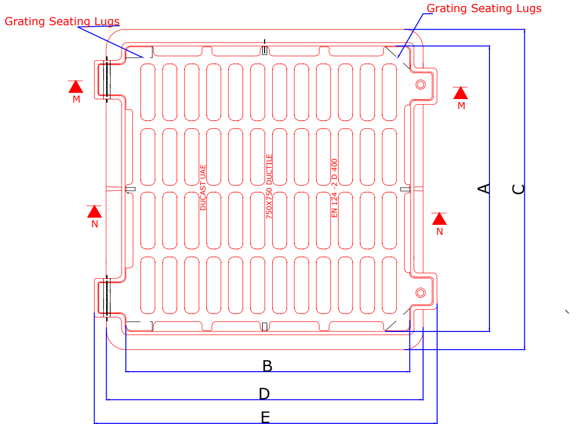
PLAN VIEW OF GRATING & FRAME
