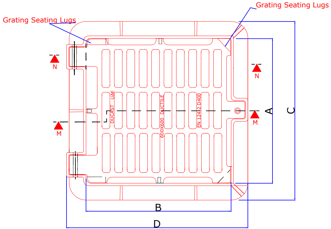
PLAN VIEW OF GRATING & FRAME
