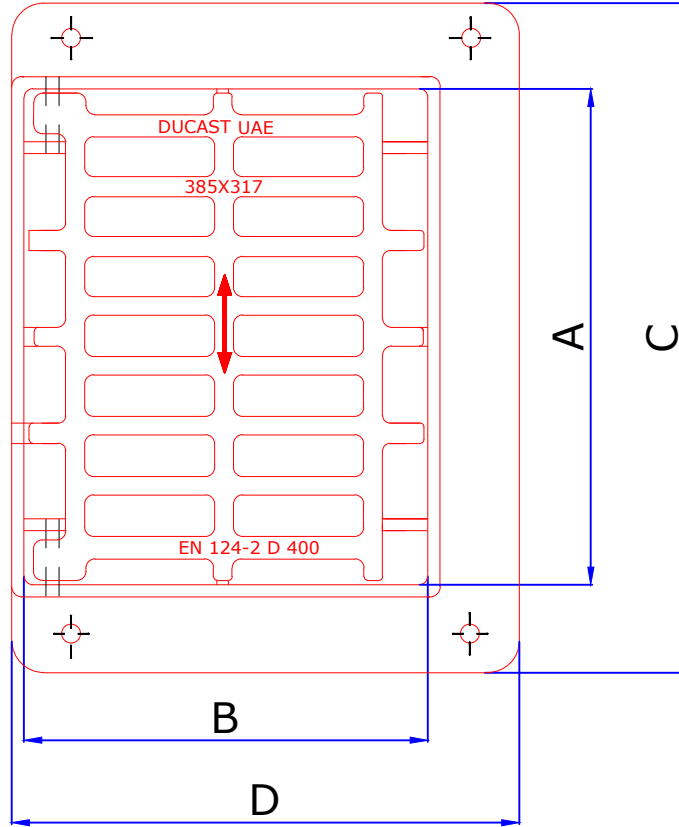
PLAN VIEW
