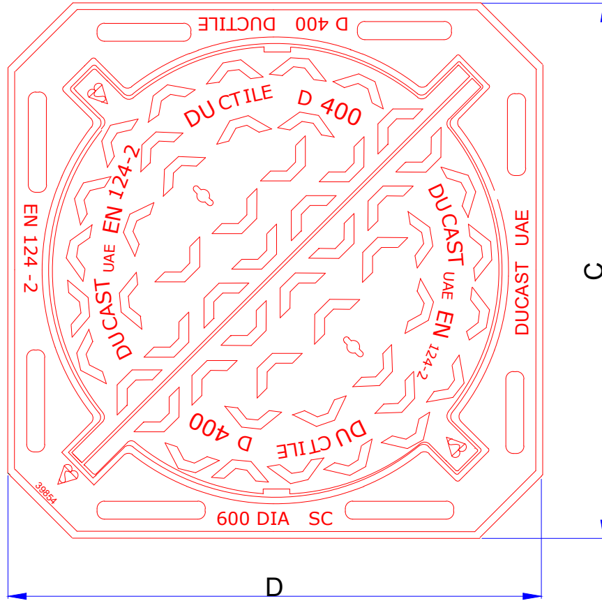
PLAN VIEW OF COVER & FRAME
