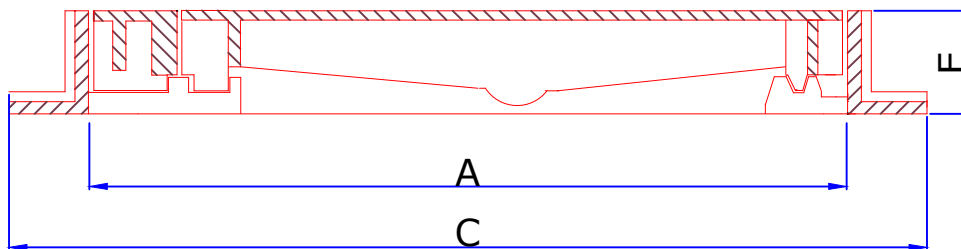
SECTIONAL VIEW
