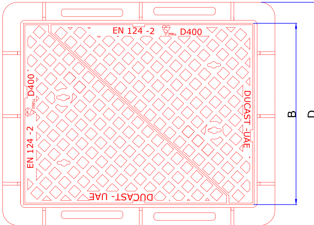
PLAN VIEW OF COVER & FRAME
