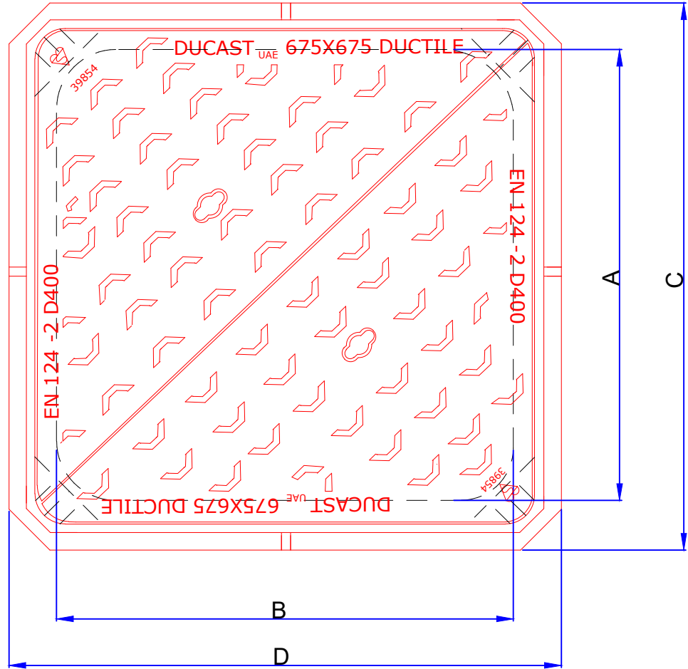
PLAN OF COVER & FRAME
