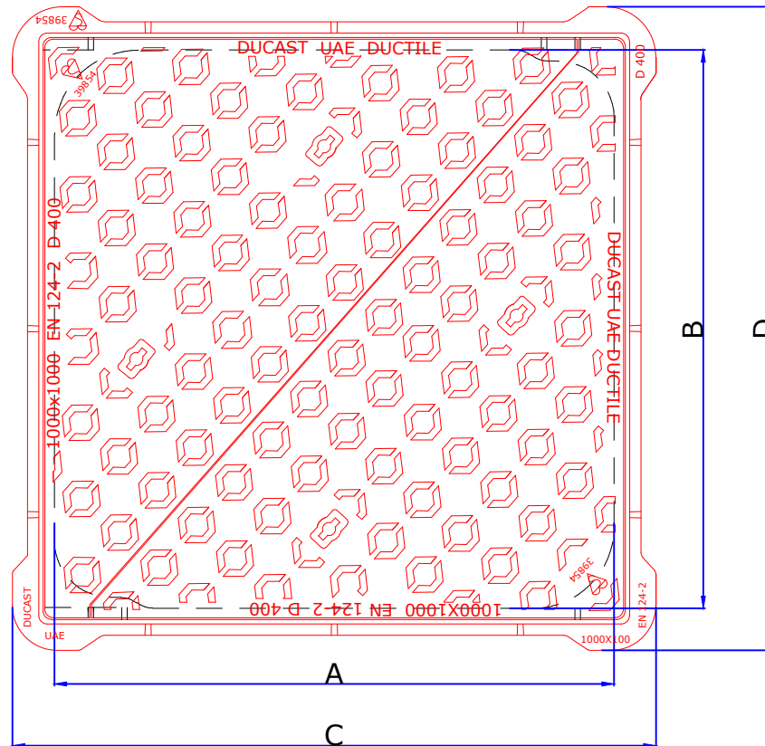
PLAN OF COVER & FRAME
