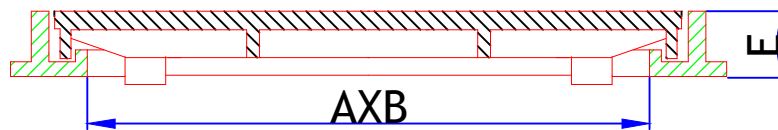
SECTIONAL VIEW
