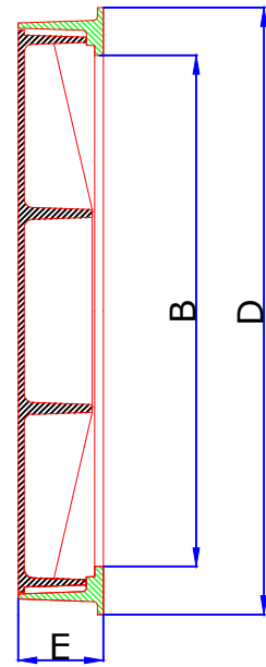
SECTION - B-B'
