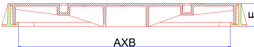
SECTION N-N
