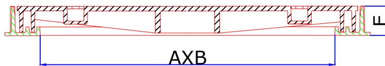
SECTION Z-Z
