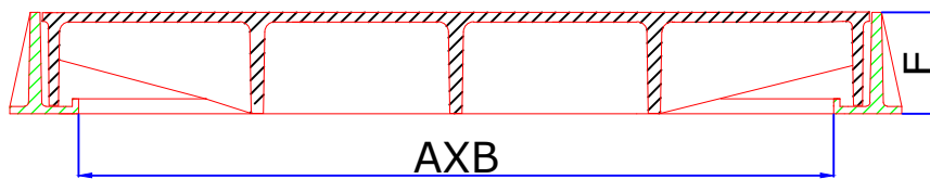
SECTION N-N
