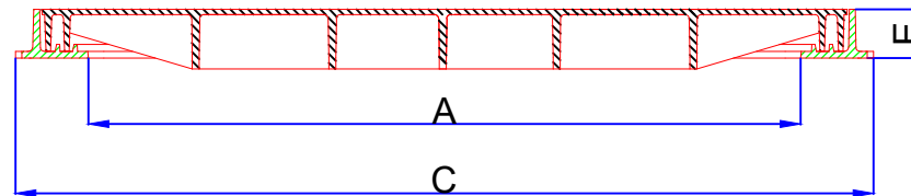
Sectional View
