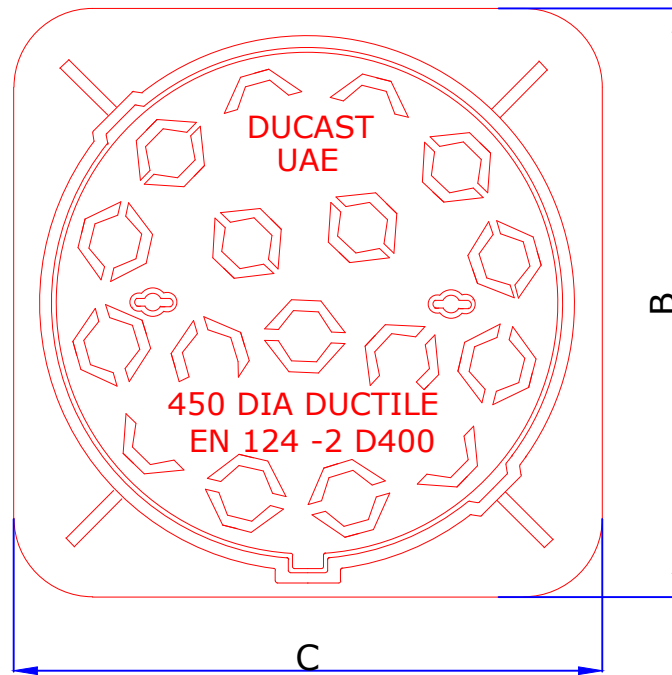
PLAN OF COVER & FRAME
