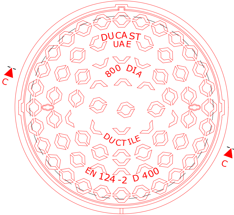
PLAN VIEW OF FRAME & COVER
