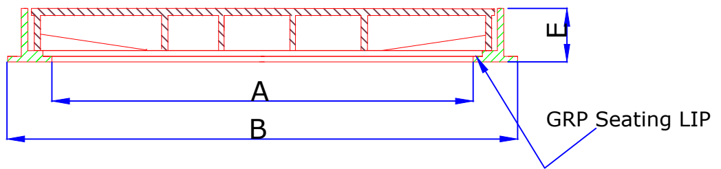
SECTION C-C
