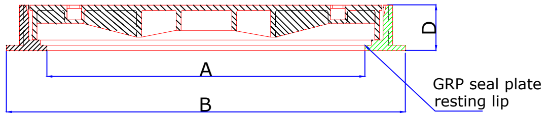
SECTIONAL VIEW
