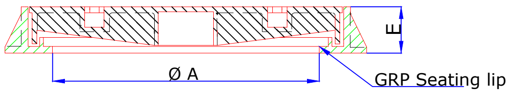
SECTIONAL VIEW
