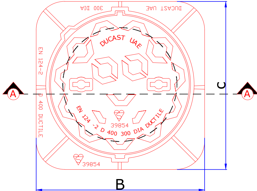
PLAN VIEW OF COVER & FRAME
