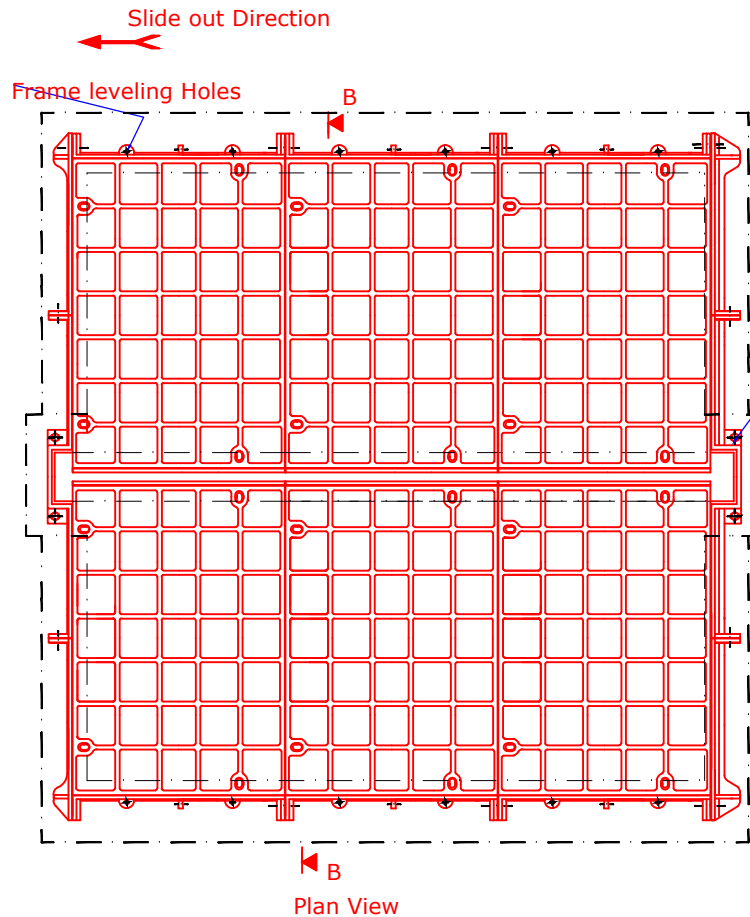
Plan View
