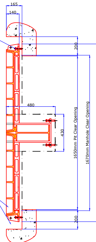
Section B-B
