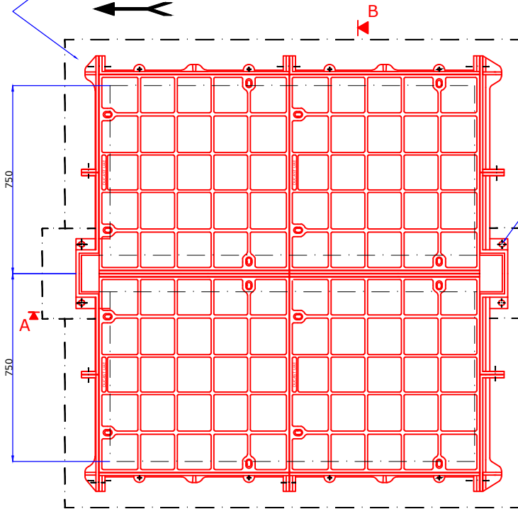
Plan View
