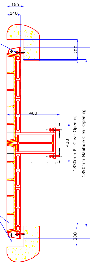
Section B-B
