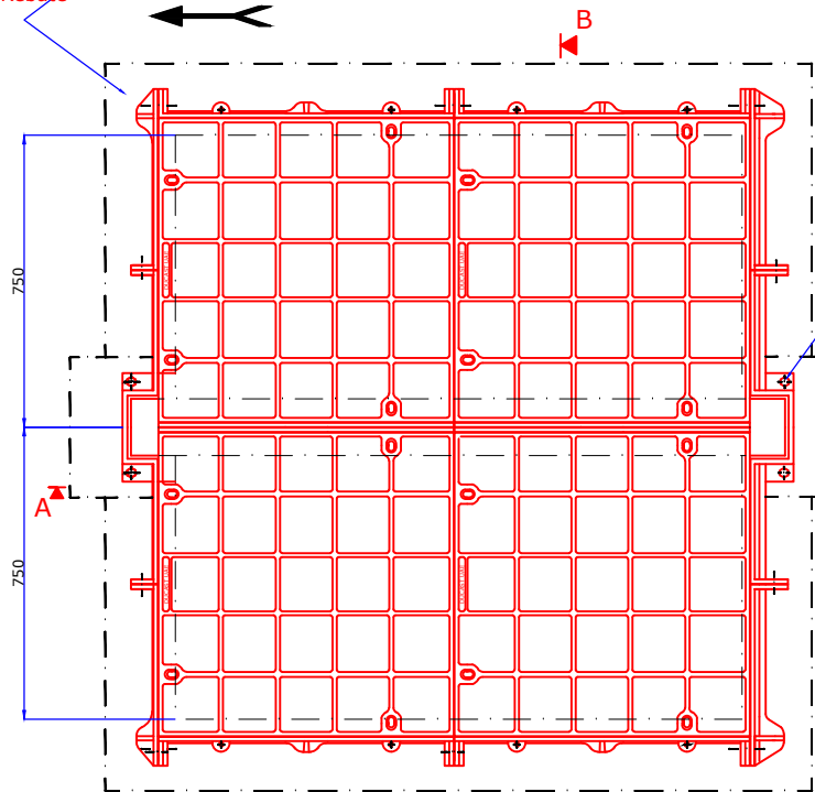
Plan View
