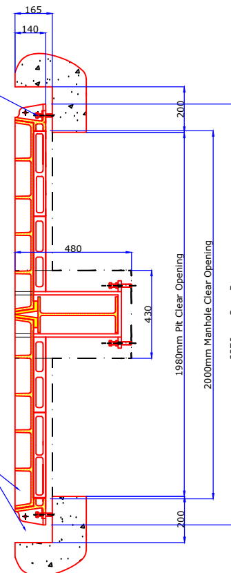
Section B-B
