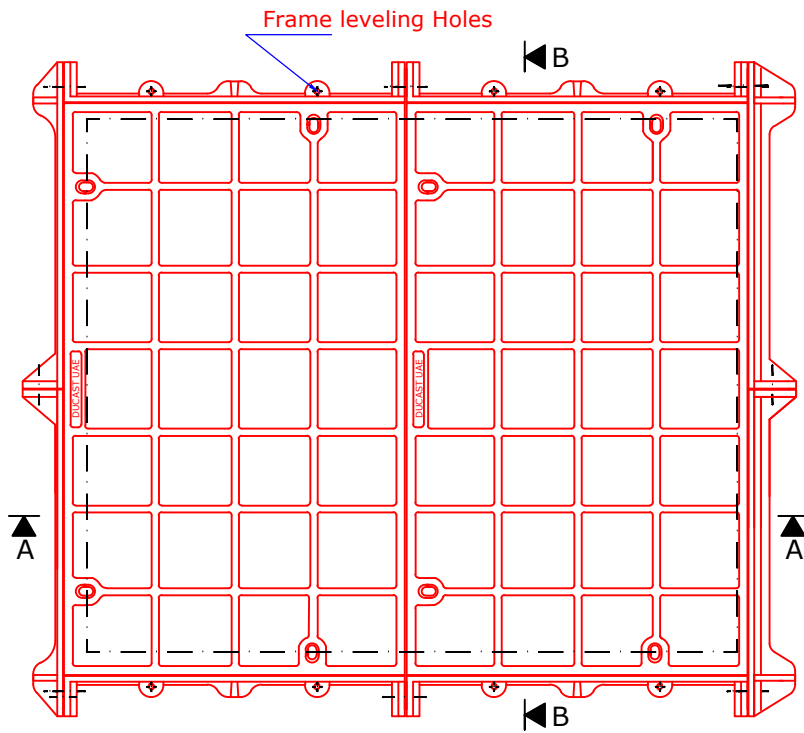
Plan View of Cover & Frame
