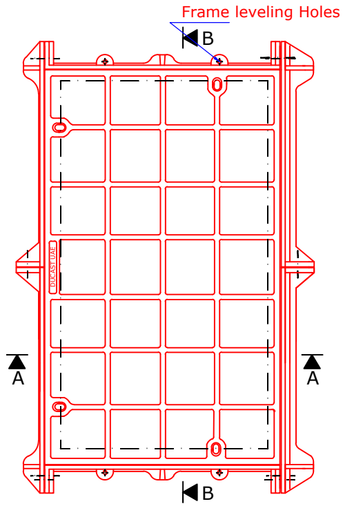
Plan View of Cover & Frame
