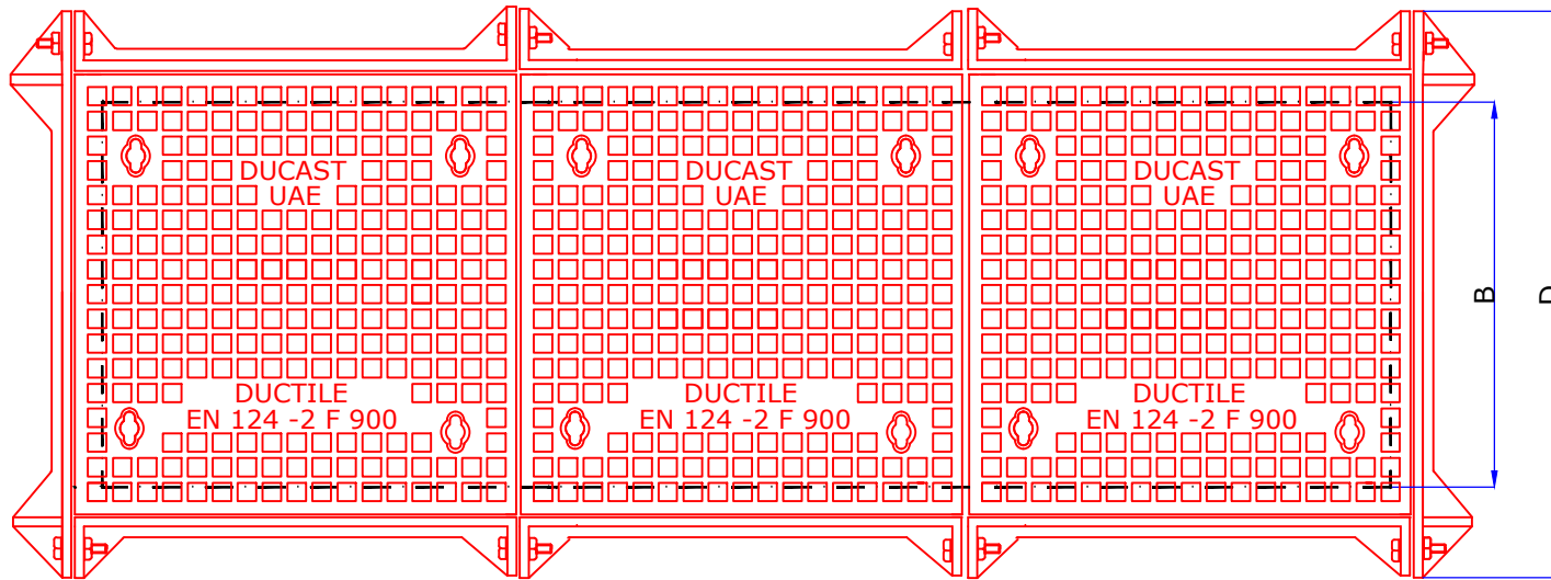
PLAN OF COVER & FRAME
