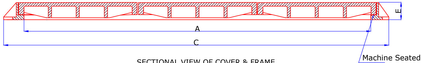
SECTIONAL VIEW OF COVER & FRAME
