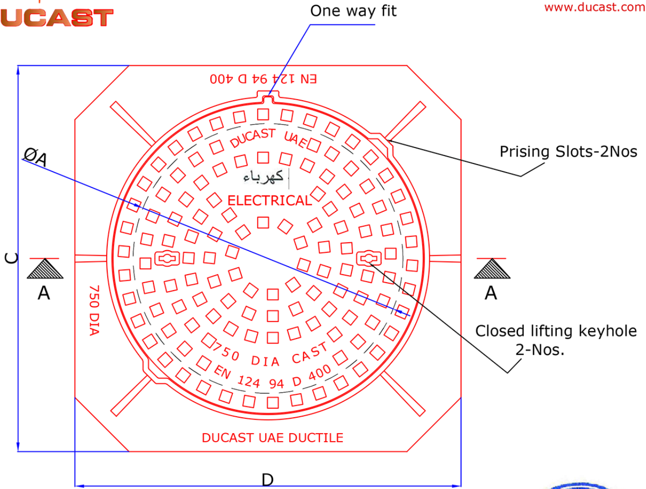
PLAN VIEW OF COVER & FRAME
