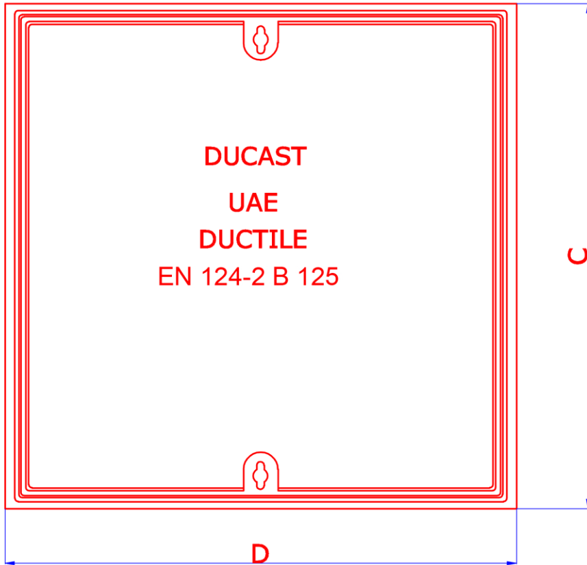
Plan View of Cover & Frame
