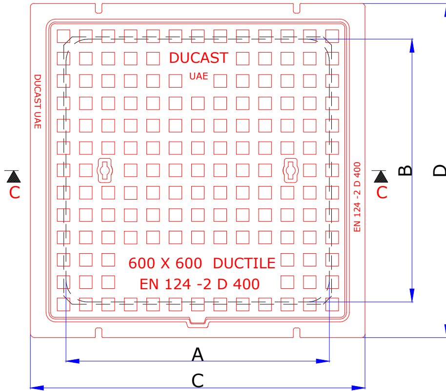
PLAN VIEW OF COVER & FRAME
