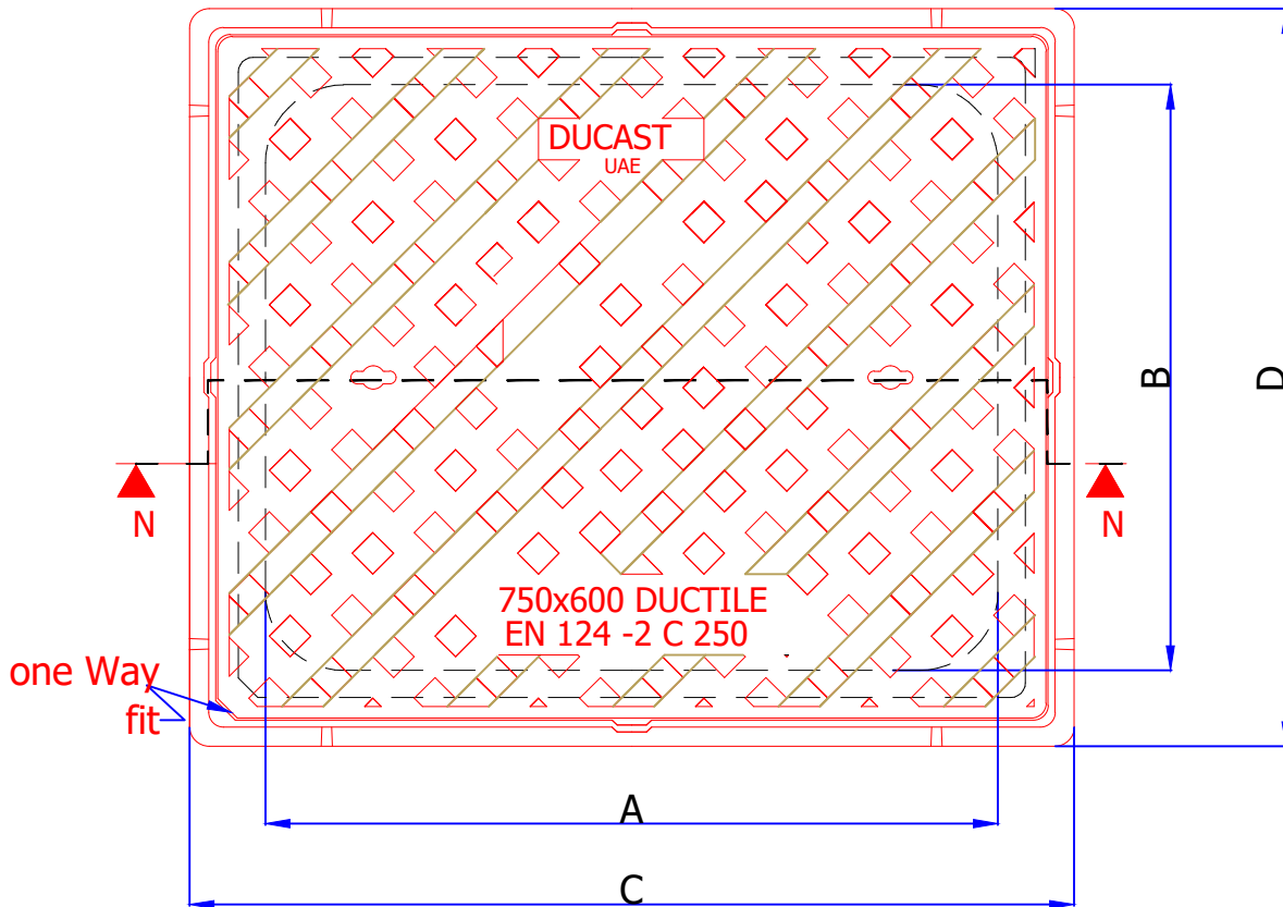
PLAN VIEW OF COVER & FRAME
