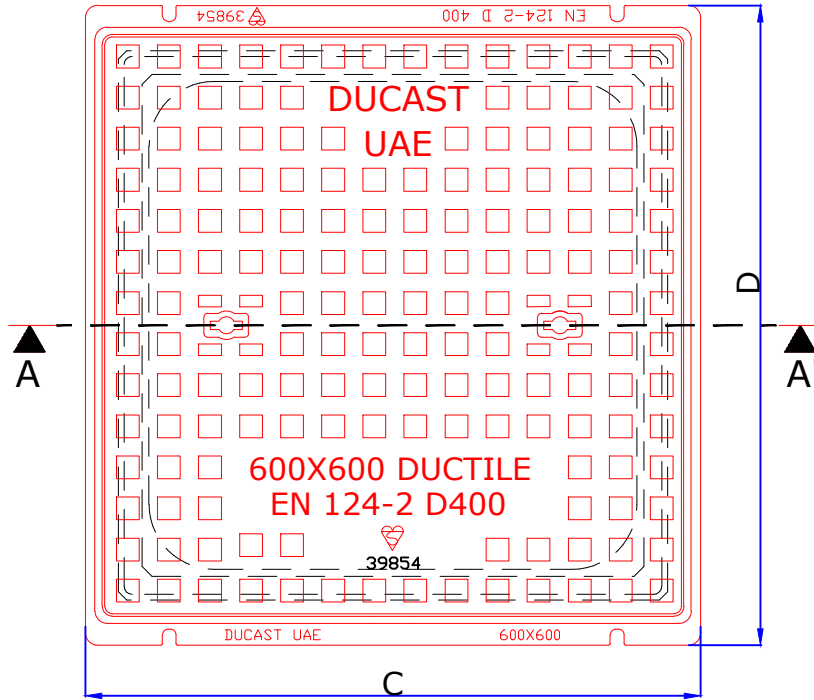
PLAN VIEW OF COVER & FRAME
