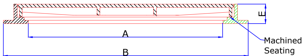
SECTIONAL VIEW OF COVER & FRAME
