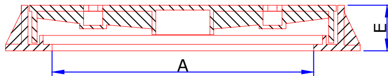
SECTIONAL VIEW OF COVER & FRAME
