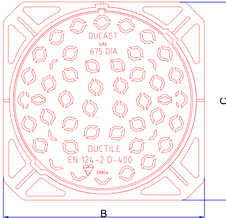
PLAN OF COVER & FRAME
